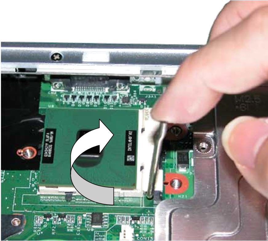
Fig. 23 Unlocking the CPU
